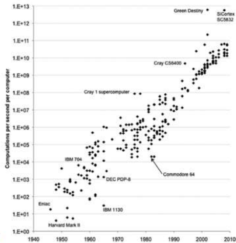
Exponentially increasing computational capacity over time (computations per second) – Koomey, Berard, Sanchez, and Wong (2011) 4
